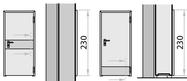
Protection plates
